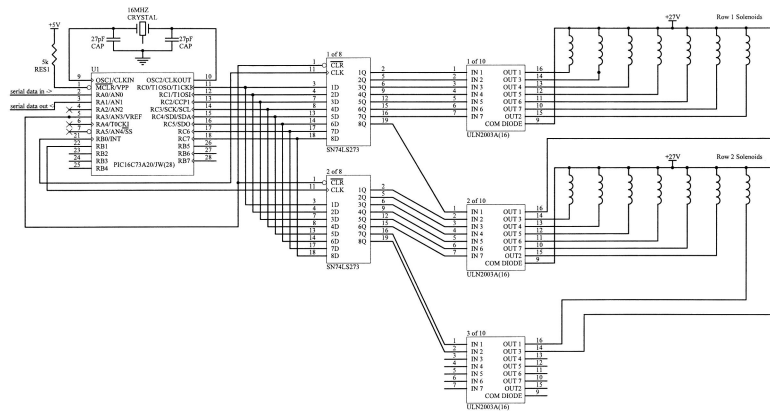
Paul Yarin's wiring diagram of the first two rows of the output hardware. A larger version of this diagram can be found in Appendix A.
