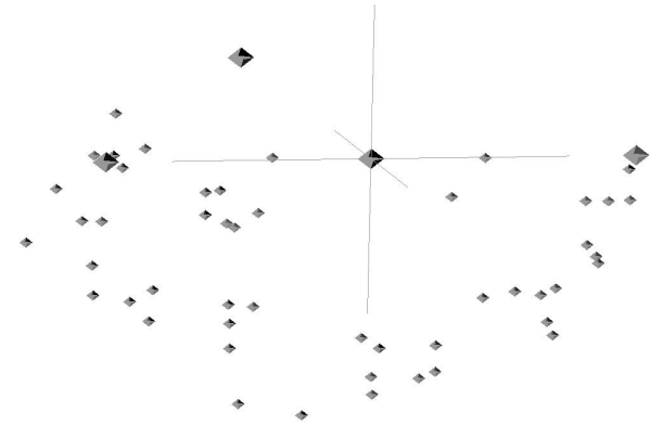
A screenshot from swarm shows particles drifting from source to sink, with no particles near the origin because the scheduler makes the region around the origin an unstable state.
